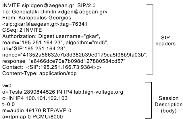
Figure 1. Well formed typical INVITE message
