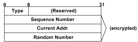
Fig.3 Format of address noticing message
