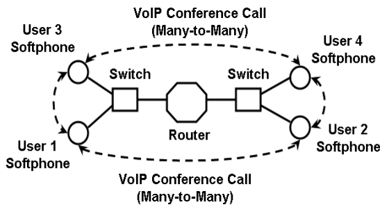
Fig. 2 VoIP over LAN Establishment: Many-to-Many (Multi Conference) Conversation
