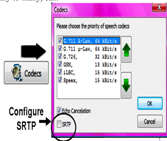
Fig. 4 3CX Softphone Codec and SRTP Configuration
